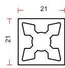
TAPS - 242 Vertical Profile
