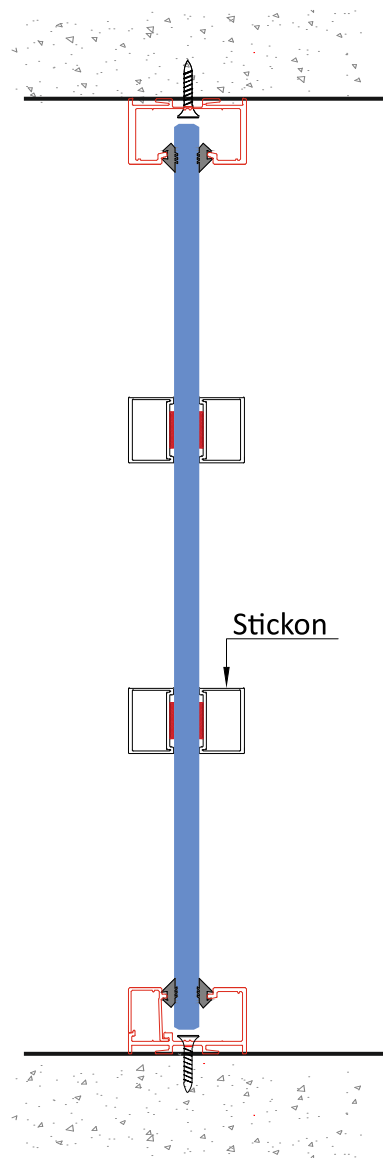
Stick-on Glazing Configuration
